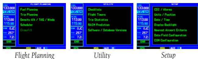
Figure 10-1 AUX Pages
